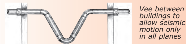
Common configuration across building expansion joints for seismic motion only in all planes
