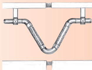
Common configuration across building expansion joints for seismic motion only in all planes
